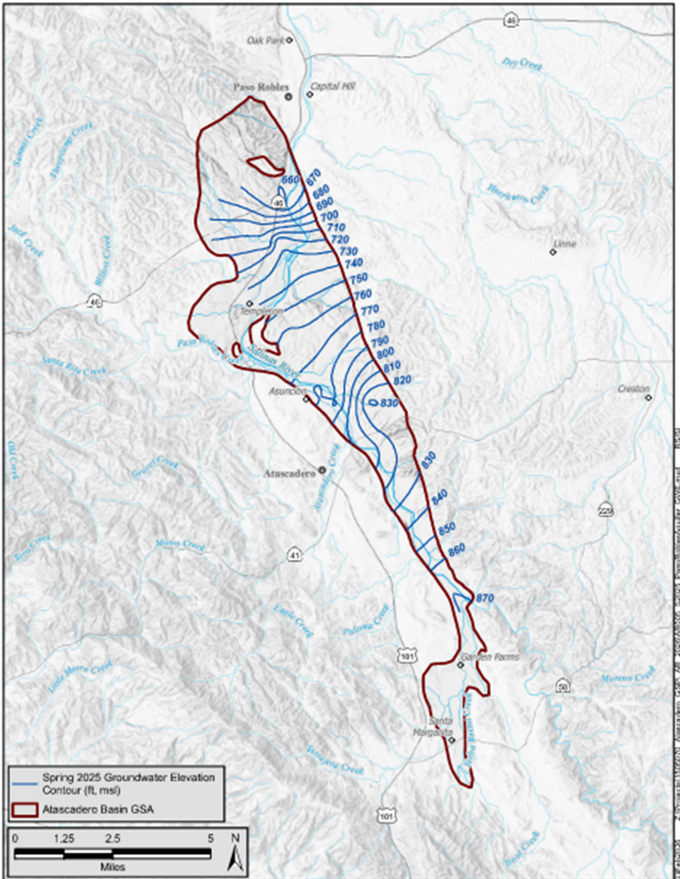
Figure 6: Paso Robles Aquifer – Groundwater Elevations Spring 2025
