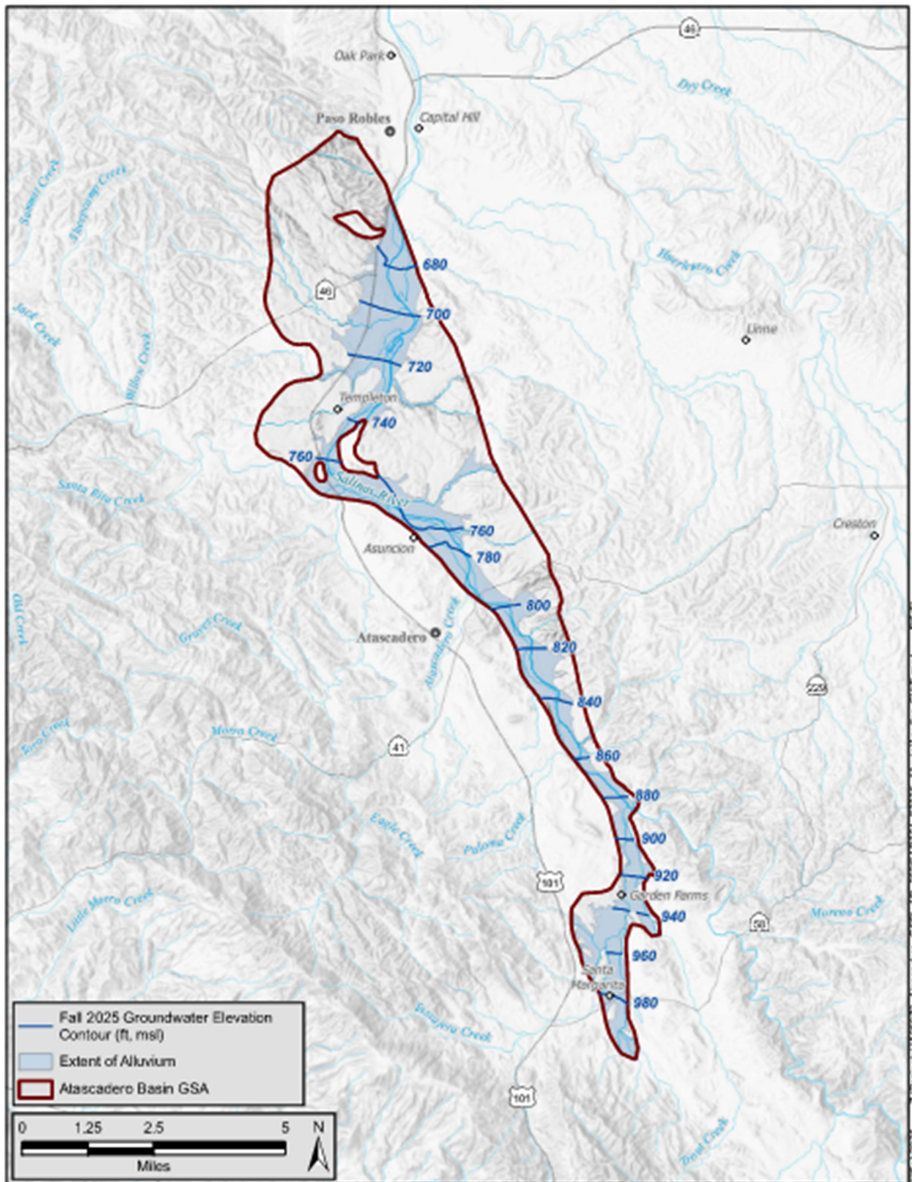
Figure 5: Alluvial Aquifer – Groundwater Elevations Fall 2025
